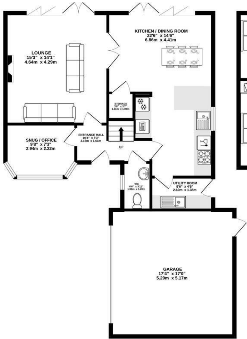
GROUND FLOOR 974 sq.ft. (90.5 sq.m.) approx.
